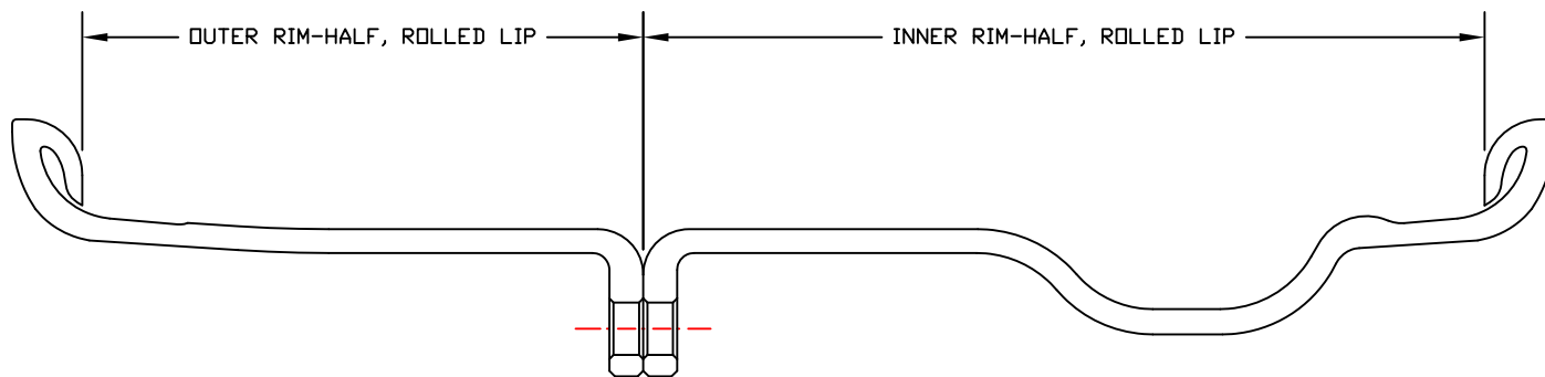
3-PIECE REVERSE CONTOUR RIM-HALVES ROLLED-LIP OUTER / ROLLED-LIP INNER
